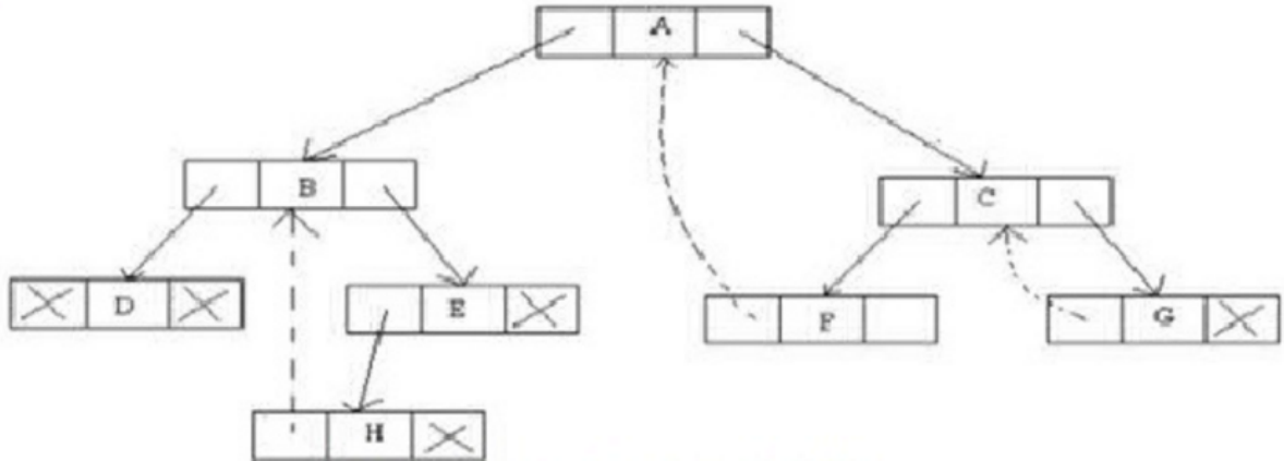
LEFT THREADED BINARY TREE
