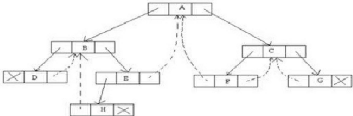
Fully Threaded Binary Tree
